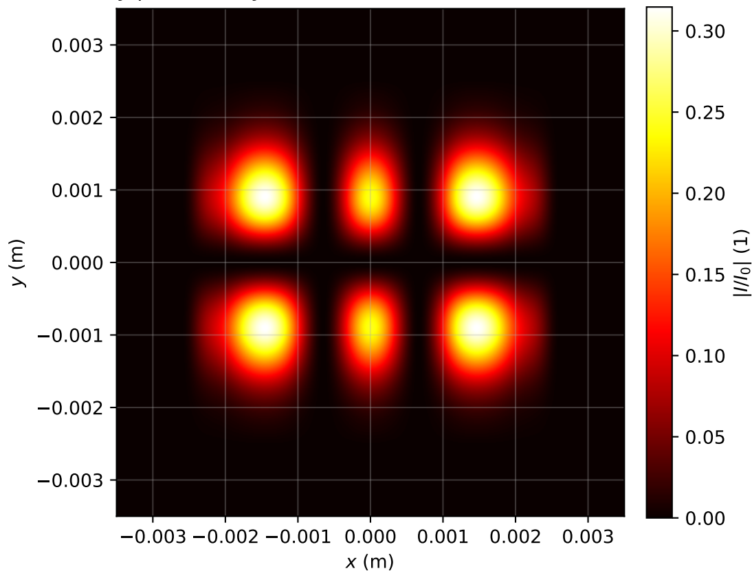
Intensity profile I(x, y, z = 3.105)/I_0 , P_{in}=0.5P_{cr} , artificial time
